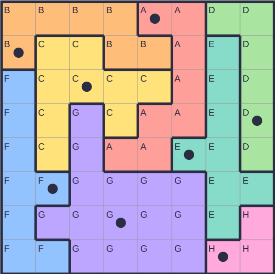
2. Star Battle 8 x 8
